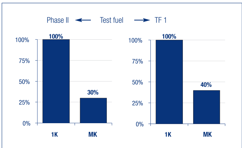
Reduced permeation achieved by means of MK connectors
